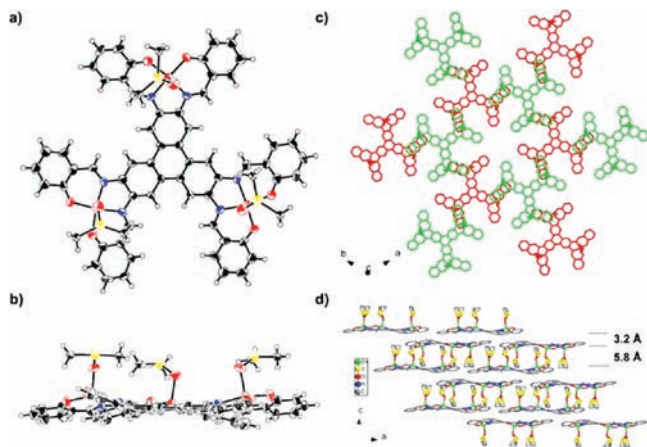
Figure 3. Crystal structure of nonalkoxylated TSZn 3 . (a) Top and (b) side views of one molecule. (c) Top and (d) side views of crystal packing. DMSO solvent coordinates with each Zn(II).
